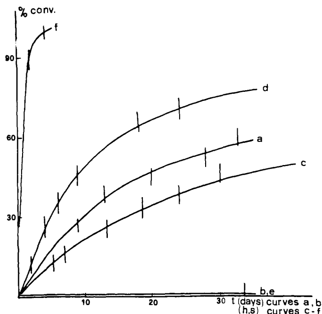
Figure 3. Conversion yields of the ASE quaternization at 37 °C in solutions of ZLI-1409 Sm B solvent (curve a) and S-1484 + ZLI-1409 nematic mixtures or S-1484 isotropic solvent (curve b). Conversion yields of the MSE quaternization in ZLI-1409 at 81 °C (curve c) and 98 °C (curve d), in isotropic or nematic solvents 1 at both temperatures (curve e). Curve f refers to MSE reactivity in its crystal phase at 81 °C.
